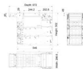
Rear service, standard throat
