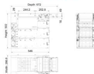
Front Service standard throat
